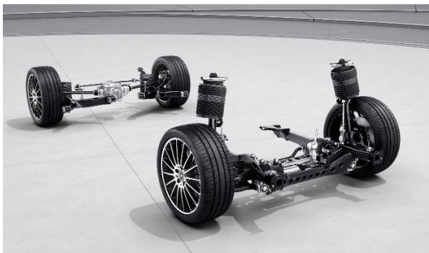
AIRMATIC - (CA4)
